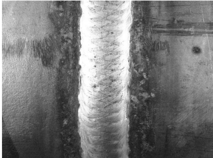
9: Plugged surface near weld joint
