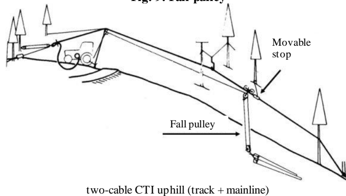
Fig. 10 Using a fall pulley at timber yarding
