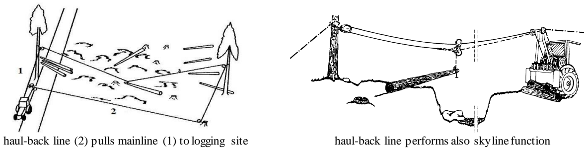
Fig. 1. Examples of adapter cable systems
