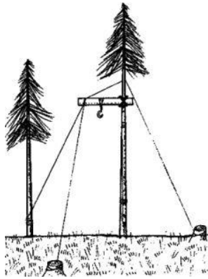
3 Fig. 53. Semi-artificial supports
