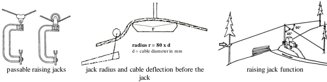
Fig. 2. Passable raising jack and its function
