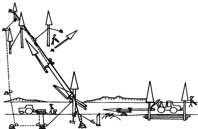
Fig. 84. Pulling trees away from the skyline integrated with delimiting using the branch-trimming unit
