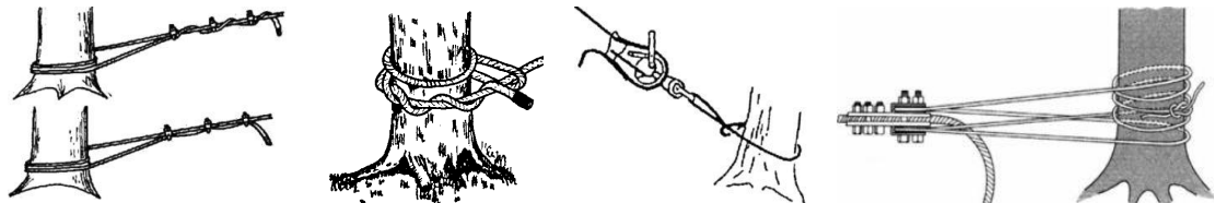
Fig. 11. Different ways of anchoring on individual trees
