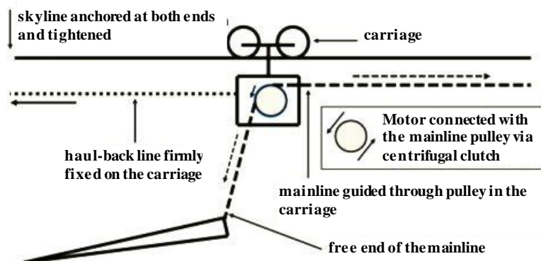
Fig. 21. Carriage with motorised extension of mainline
