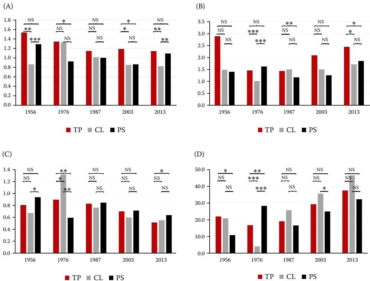
Figure 12. Graph of resilience indices: (A) resilience, (B) recovery, (C) resistance and (D) average relative growth reduction *P < 0.05 ; **P < 0.01 ; ***P < 0.001 ; NS – non-significant; TP – western redcedar ( Thuja plicata ); CL – Lawson cypress ( Chamaecyparis lawsoniana ); PS – Scots pine ( Pinus sylvestris )
