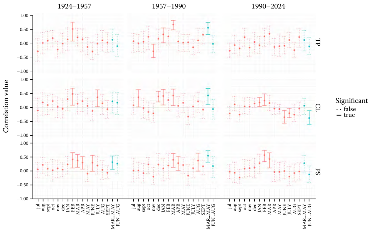
Figure 8. Pearson's correlation coefficients between tree ring indices and mean monthly temperature
