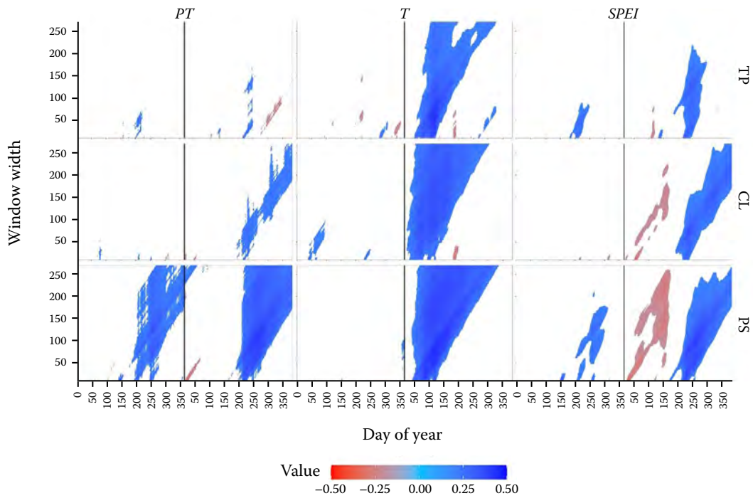
Figure 10. Heatmap of daily Pearson correlation coefficients between tree-ring indices and daily climate characteristics of precipitation ( PT ), air temperature ( T ) and standardised precipitation evapotranspiration index ( SPEI )
