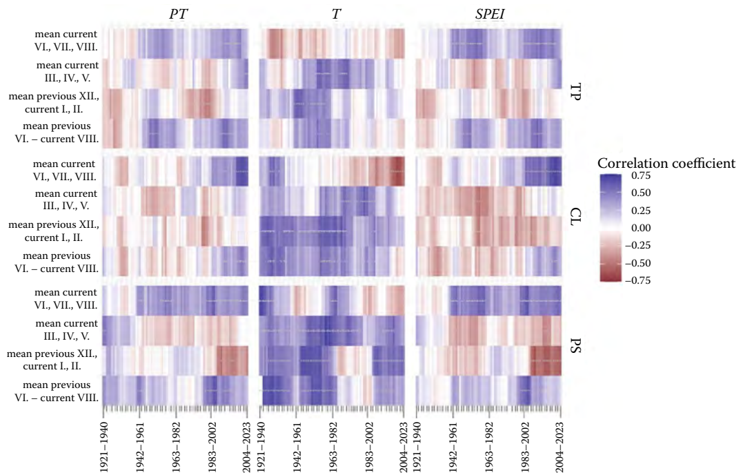
Figure 11. Moving Pearson correlation coefficients between tree-ring and monthly climate characteristics of precipitation ( PT ), temperature ( T ) and standardised precipitation evapotranspiration index ( SPEI )
