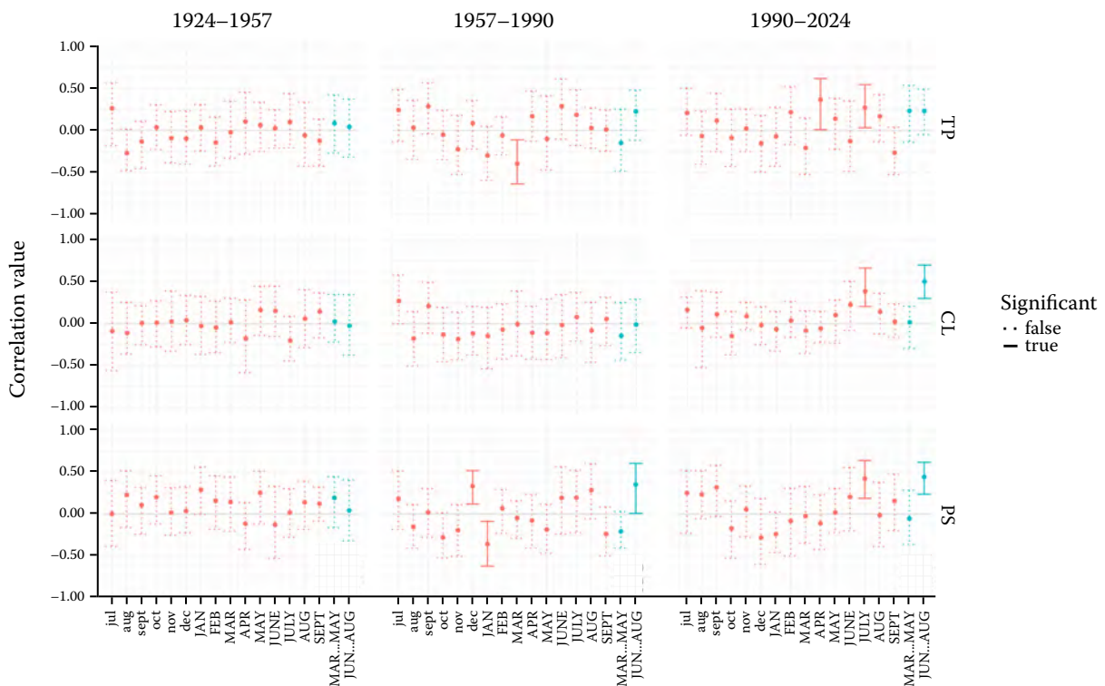
Figure 7. Pearson's correlation coefficients between tree ring indices and monthly precipitation
