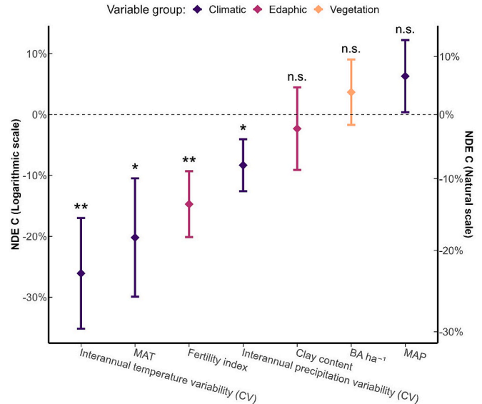
Fig. 3. Standardized effects of climatic, edaphic, and vegetation variables on the net diversity effect on topsoil C stocks (NDE C) across nine sites ( n = 110 ) on a logarithmic scale (first y-axis; left) and natural scale (second y-axis; right). Error bars denote standard errors. Climatic variables include mean annual temperature (MAT), mean annual precipitation (MAP), as well as variability in temperature and precipitation (interannual CV). Edaphic variables include the inverted first principal component axis for soil pH and C:N ratio (Fertility index) as well as soil texture (based on clay content). Effects of standing stock is represented by basal area per hectare (BA ha -1 ). Significant effects on NDE C are indicated as *** = p < 0.001 , ** = p < 0.01 , * = p < 0.05 , n.s. = not significant. Values below 0 indicate negative correlation between NDE C and predictors.
